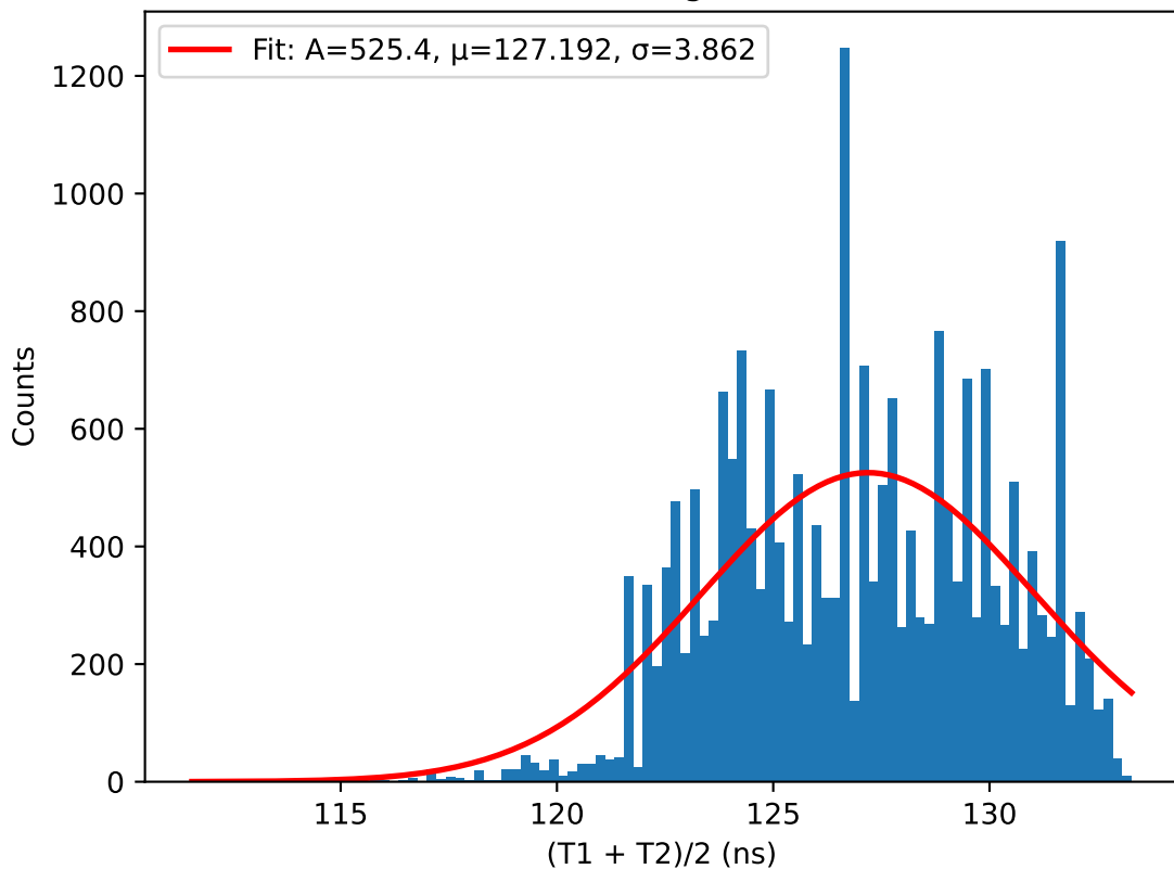
(T1 + T2)/2 histogram for 43.5V
