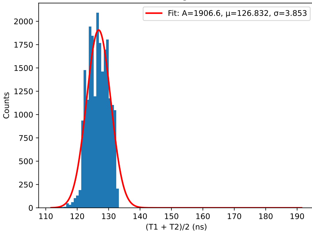
(T1 + T2)/2 histogram for 42.0V
